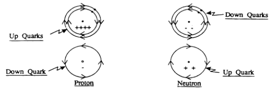
Fig. 7 The stacked-interactions and the electromagnetic interactions in a proton and a neutron.
